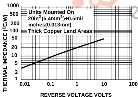
Fig. 5-TRANSIENT THERMAL IMPEDANCE
